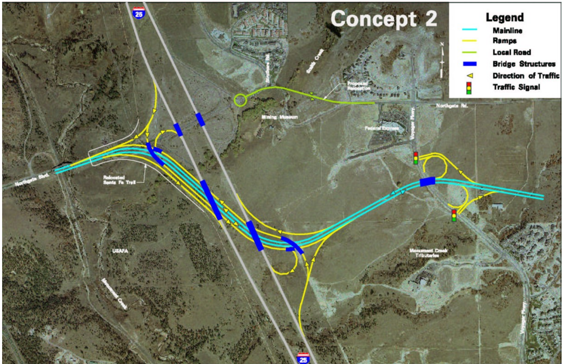
FIGURE 9-5 Concept 2: Realign Air Force Academy Entrance to Meet Powers South at a New Interchange
