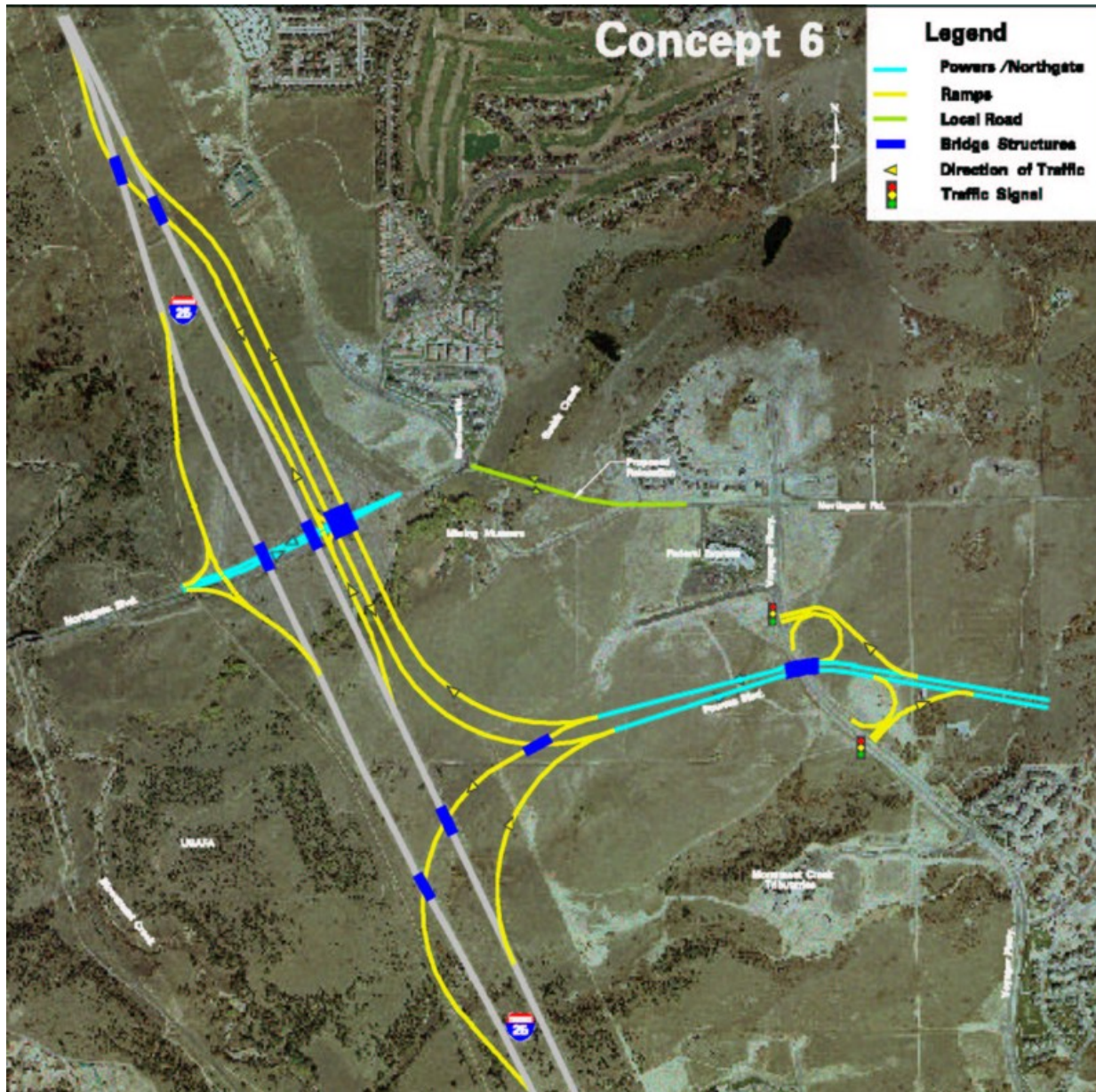
FIGURE 9-9 Concept 6: Powers Alignment East of I-25 with North Connection at Diamond Interchange at North Gate
