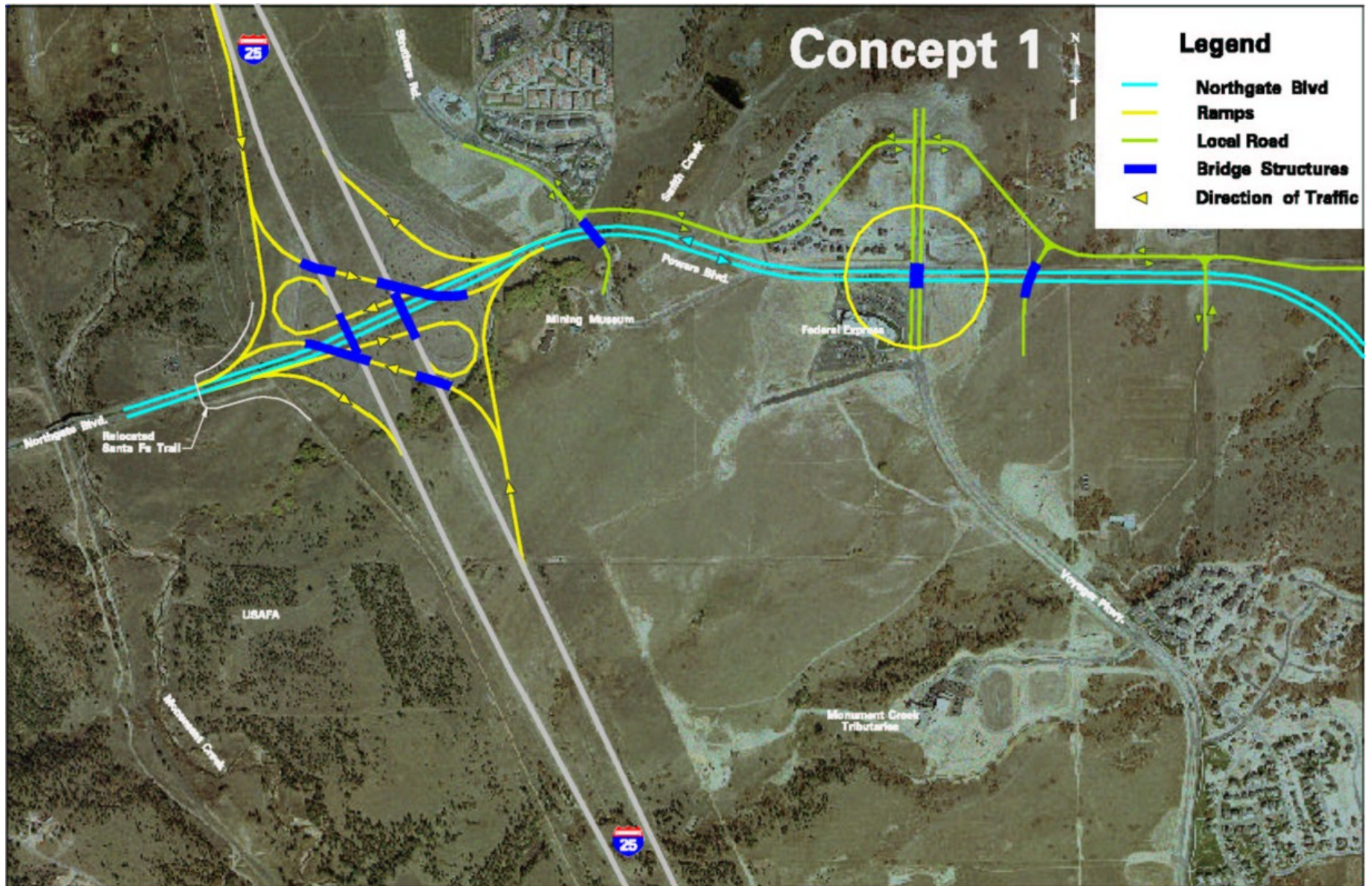
FIGURE 9-4 Concept 1: Realign Powers Along North Gate Boulevard to Improved North Gate Interchange
