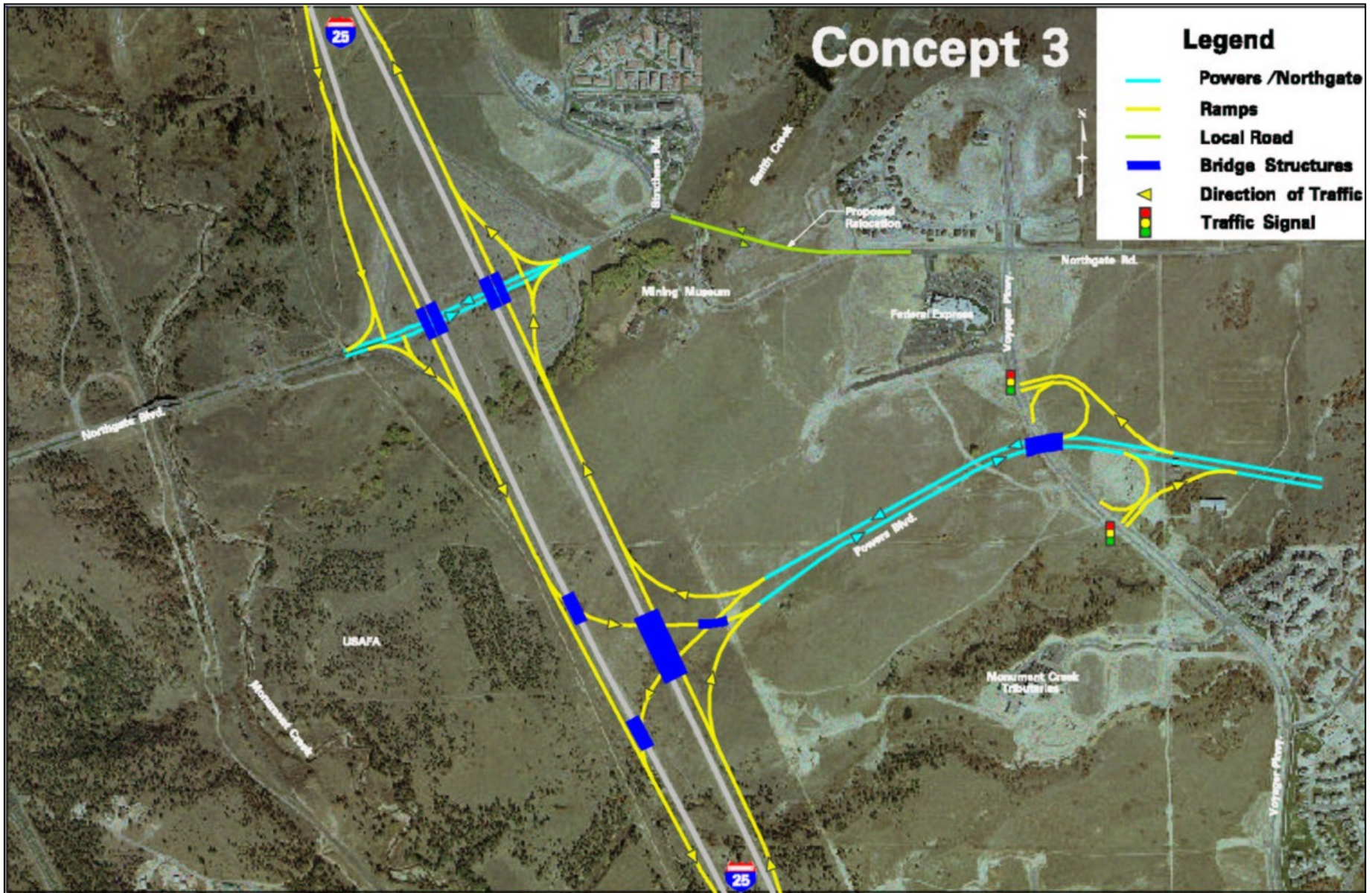
FIGURE 9-6 Concept 3: Collector/Distributor Roads with Diamond Interchange at North Gate and New Powers Connection
